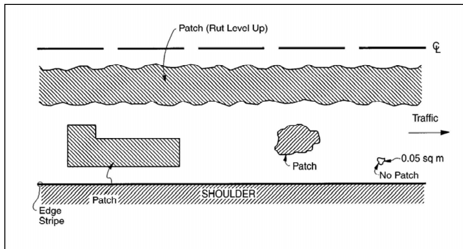
FIGURE 13: Patching Variations
