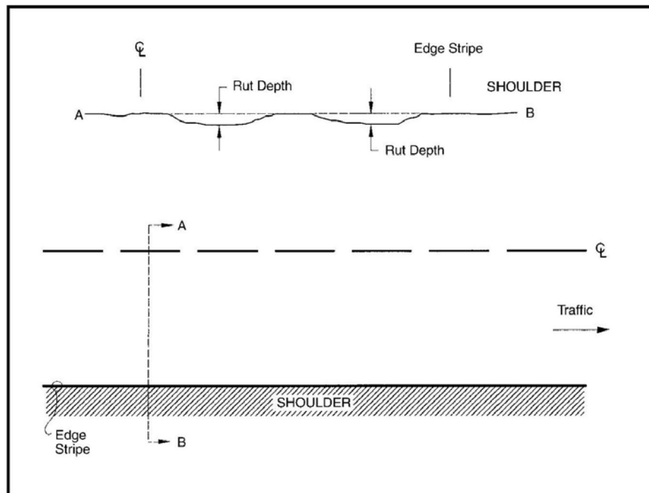
FIGURE 18: Measuring Rutting
