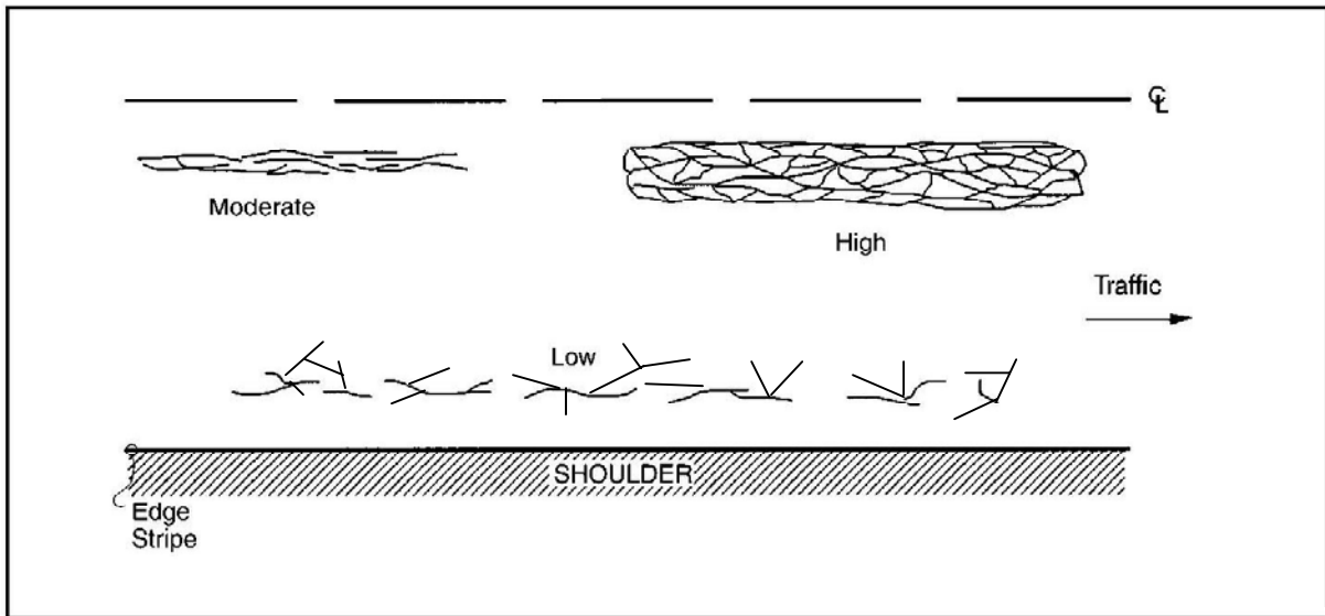
FIGURE 3: Alligator Crack Patterns of Differing Severity
