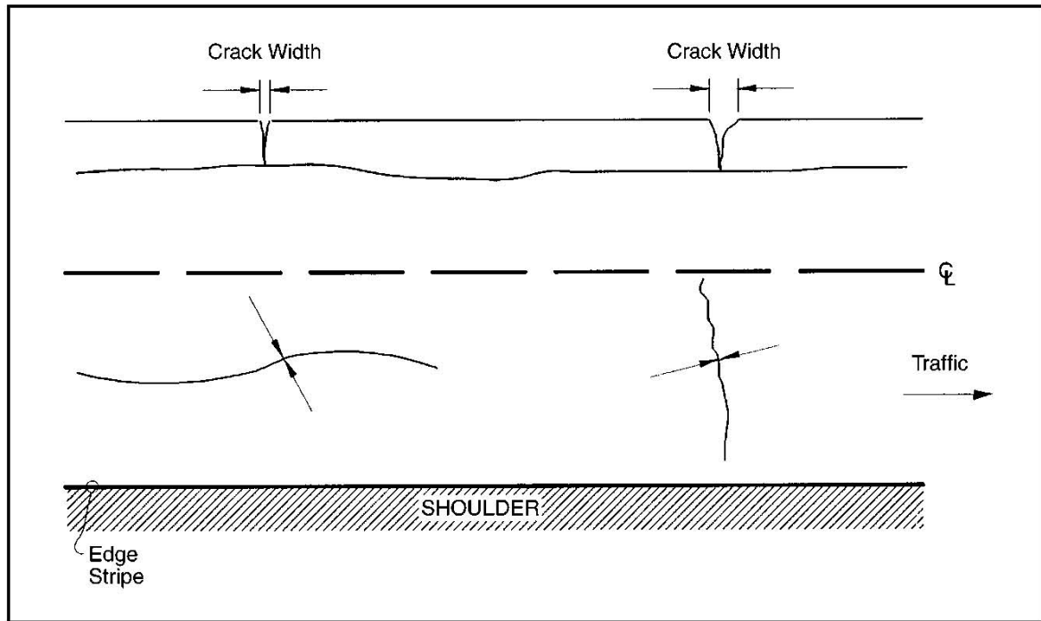
FIGURE 1: Measuring Crack Width on Asphalt Pavement
